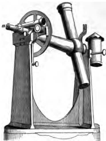
THE CARSHALTON TRANSIT.
